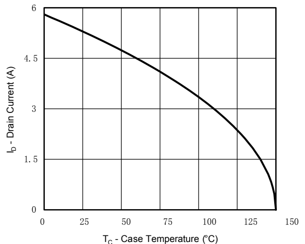
Current Derating*
